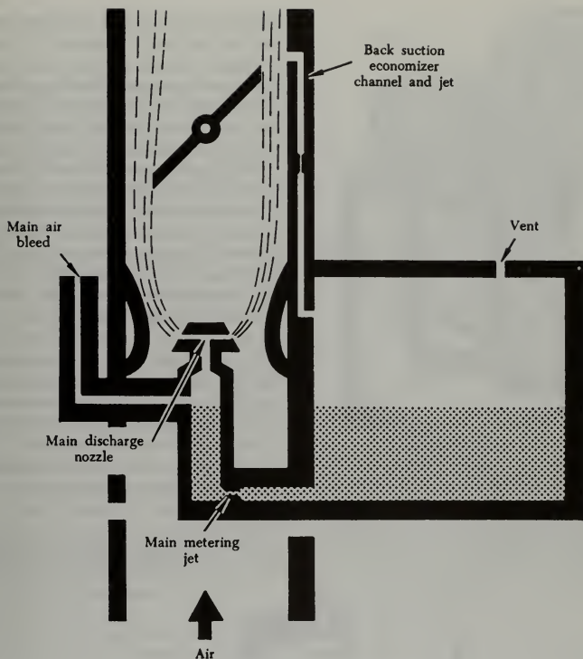
FIGURE 3-16. Back-suction economizer system.
